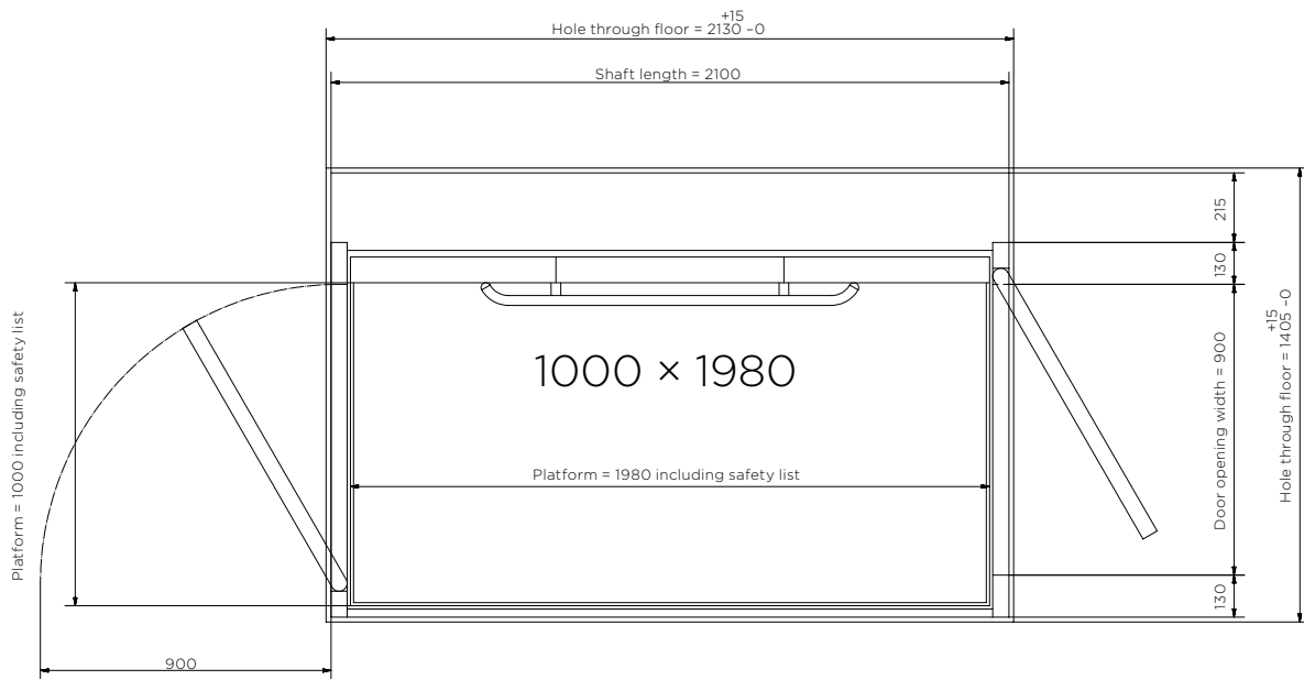
Platform 1000 × 1980
