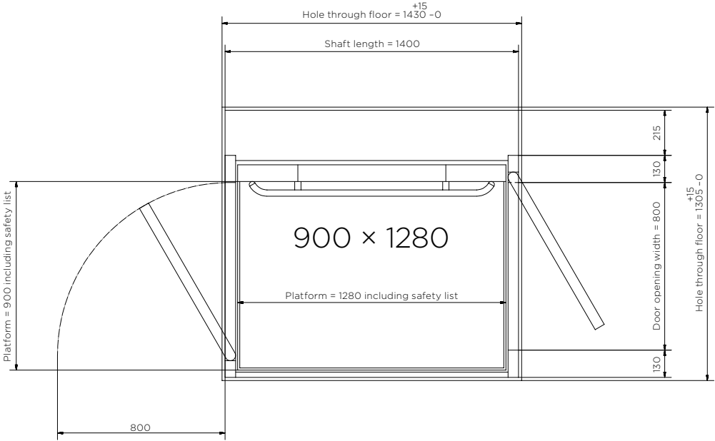
Platform 900 × 1280
