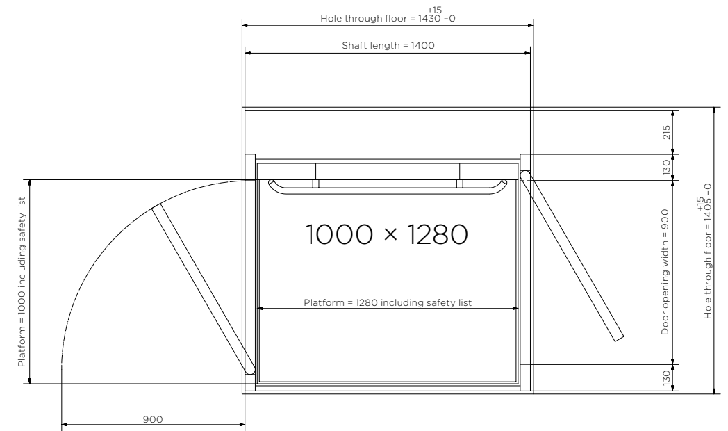
Platform 1000 × 1280
