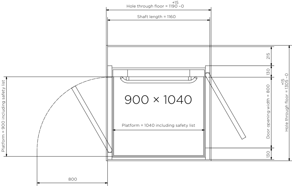
Platform 900 × 1040
